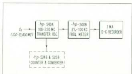
Fig. 10. Set-up for recording drifts in frequencies in 100-12,400 mc range.
